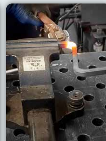
STEEL BAR BENDING - CINTRAGE BARRE ACIER
