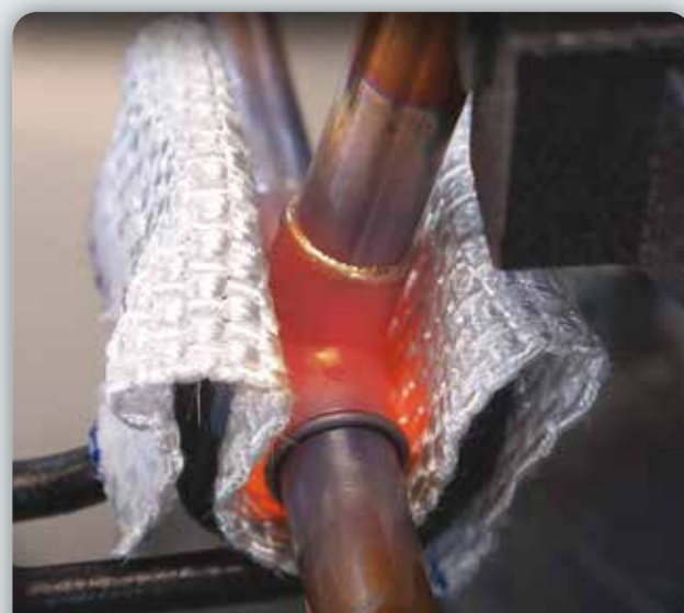
BRAZING COPPER FITTING - BRASAGE RACCORD CUIVRE
