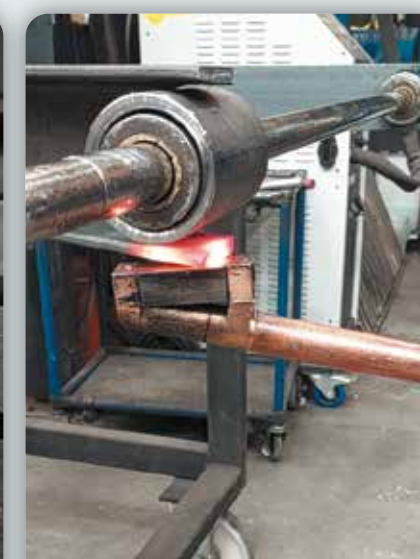
TRAILER MANUFACTURE - STEEL BENDING - FABRICATION DE REMORQUE - CINTRAGE ACIER
