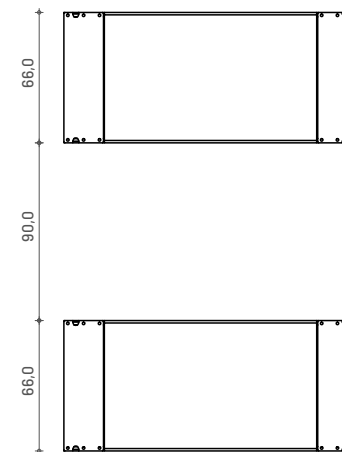
DIMENSIONS AND RECESS INSTALLATION DRAWING DM4.OPRO DIMENSIONS = cm
