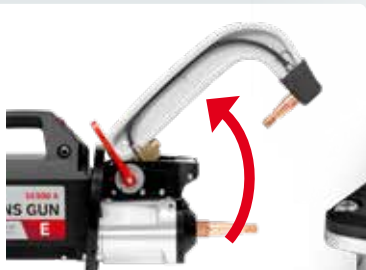
Easy opening Ideal for difficult access Ultra fast arm switching
