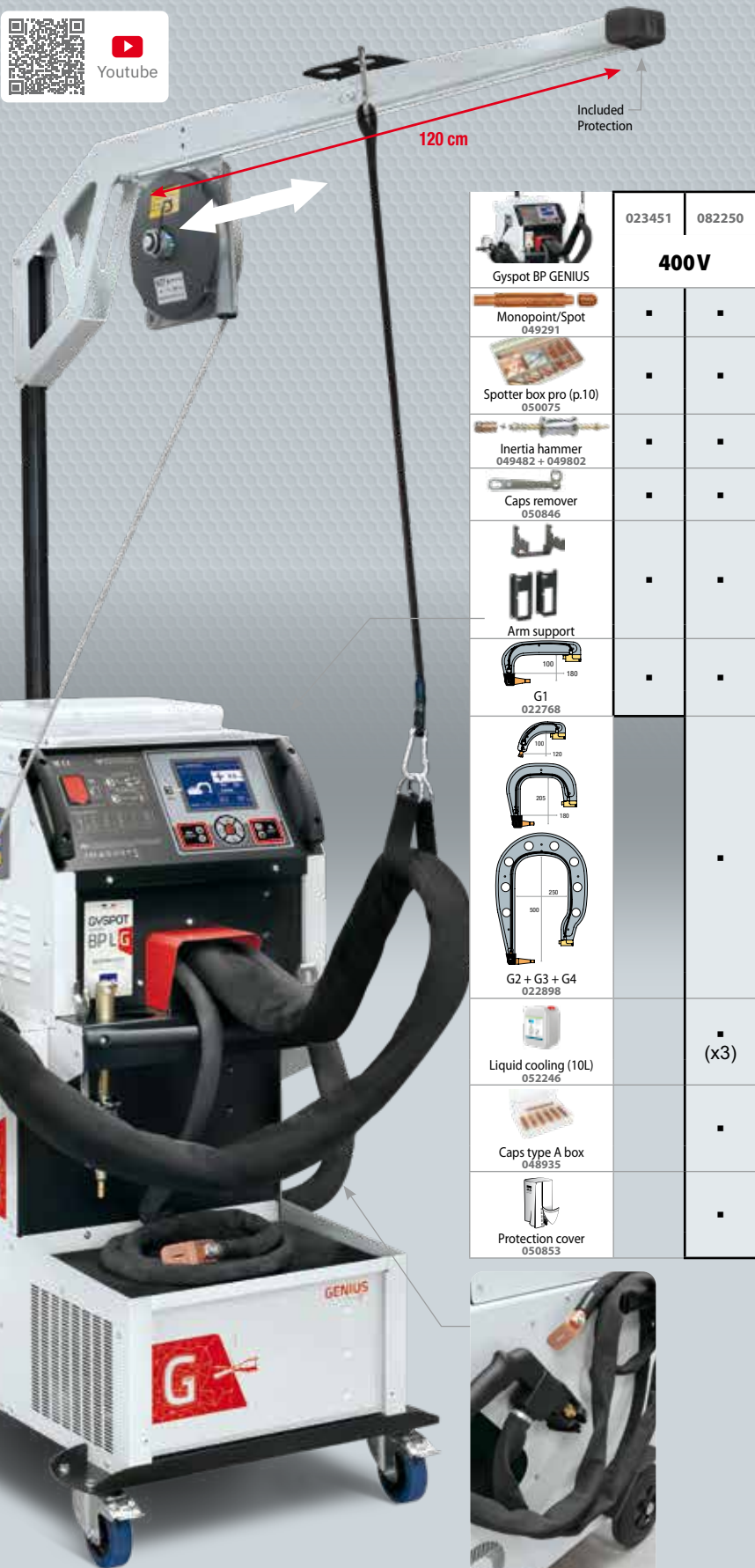
Gun & cable support
